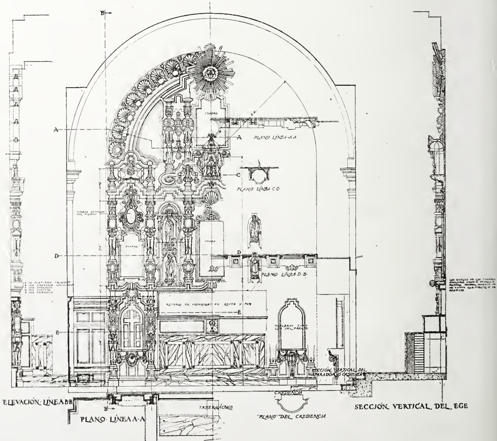
ALTAR AND REREDOS—TRINITY CHURCH.
